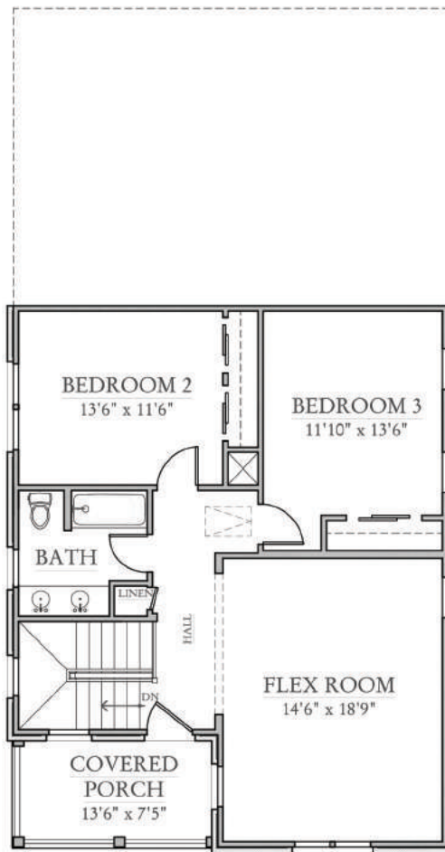
SECOND FLOOR - OPTIONAL FLEX ROOM
