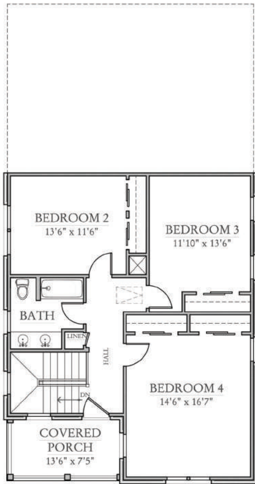
SECOND FLOOR - OPTIONAL BEDROOM
