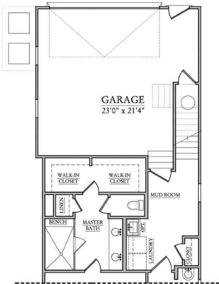
OPT. BONUS ROOM AT FIRST FLOOR
